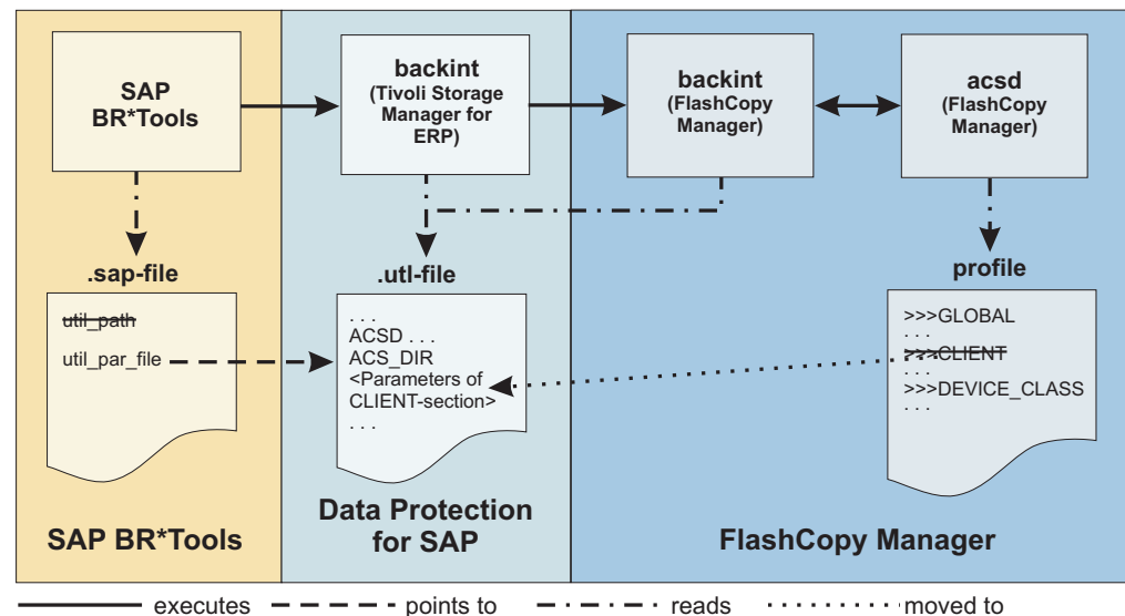
Figure 16. SAP with Oracle, Tivoli Storage FlashCopy Manager with Tivoli Storage Manager
